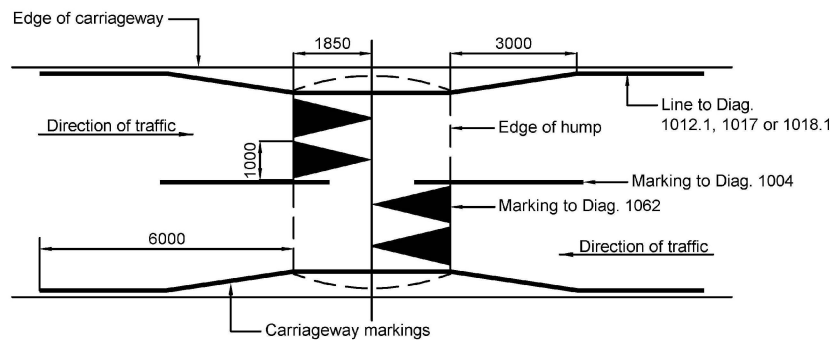
PLAN SHOWING LINING
