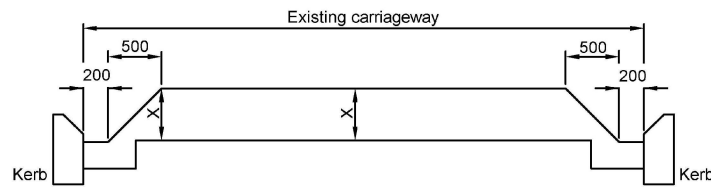
CROSS SECTION
