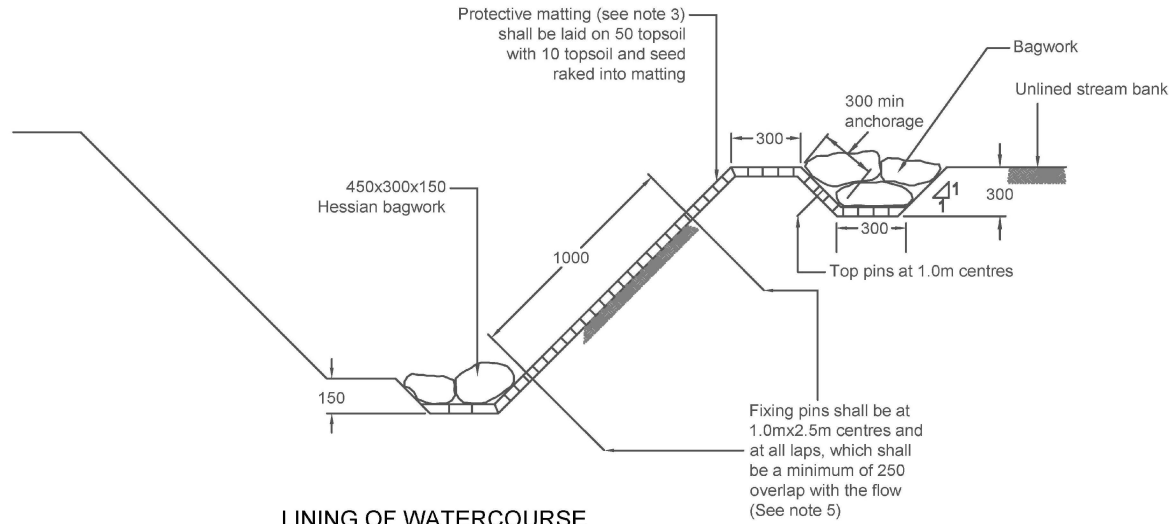
LINING OF WATERCOURSE
