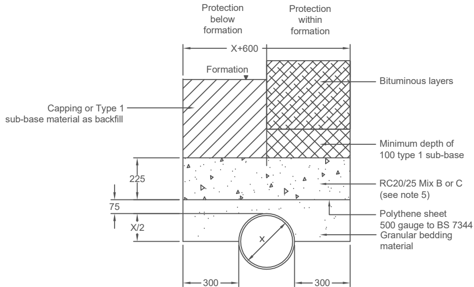
PROTECTION TO EXISTING PIPES OR DUCTS
