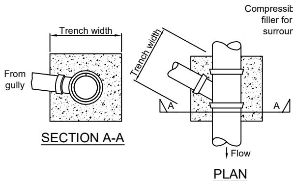
GULLY CONNECTION DETAILS
