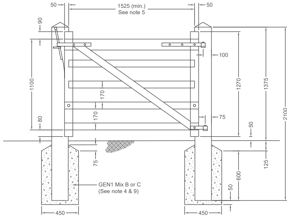
PEDESTRIAN/BRIDLE TIMBER FIELD GATE
