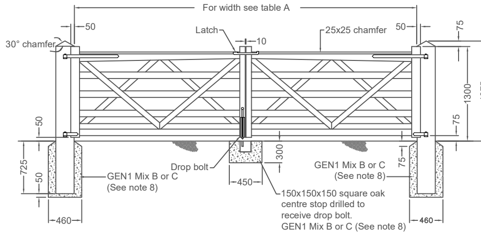
DOUBLE LEAF FIELD GATE TYPE A
