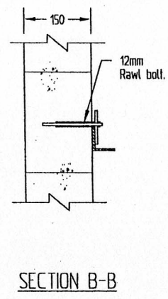
GRID FRAME (fixing detail)
