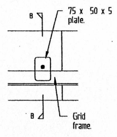
GRID FRAME (fixing detail)
