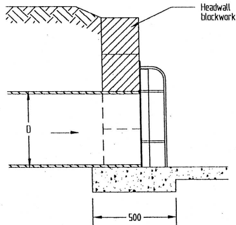
SECTION OF GRID AS POSITIONED ON HEADWALL
