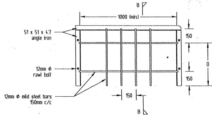
FRONT ELEVATION OF GRID
